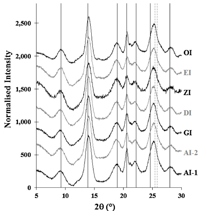
Fig. 3. X-ray diffraction patterns of examples of all monofragment isoforms, displaced vertically to separate them. The seven vertical solid lines are at 2\theta values calculated (Bragg's law) from the d_{\text{obs}} spacings of the monohydrate inulin crystal reported by André, Putaux, et al. (1996, Table 4: hkl designations 101, 111/201, 202/112, 020/310, 311/021, 400/220, and 222/402, of which six values are composites of more than one diffraction peak). The peak at \sim 25.5^\circ 2\theta is taken to be a composite of d_{\text{obs}} spacings 400/220, and 221/411 (dashed lines) from electron diffraction data in Table 3 of that paper.
