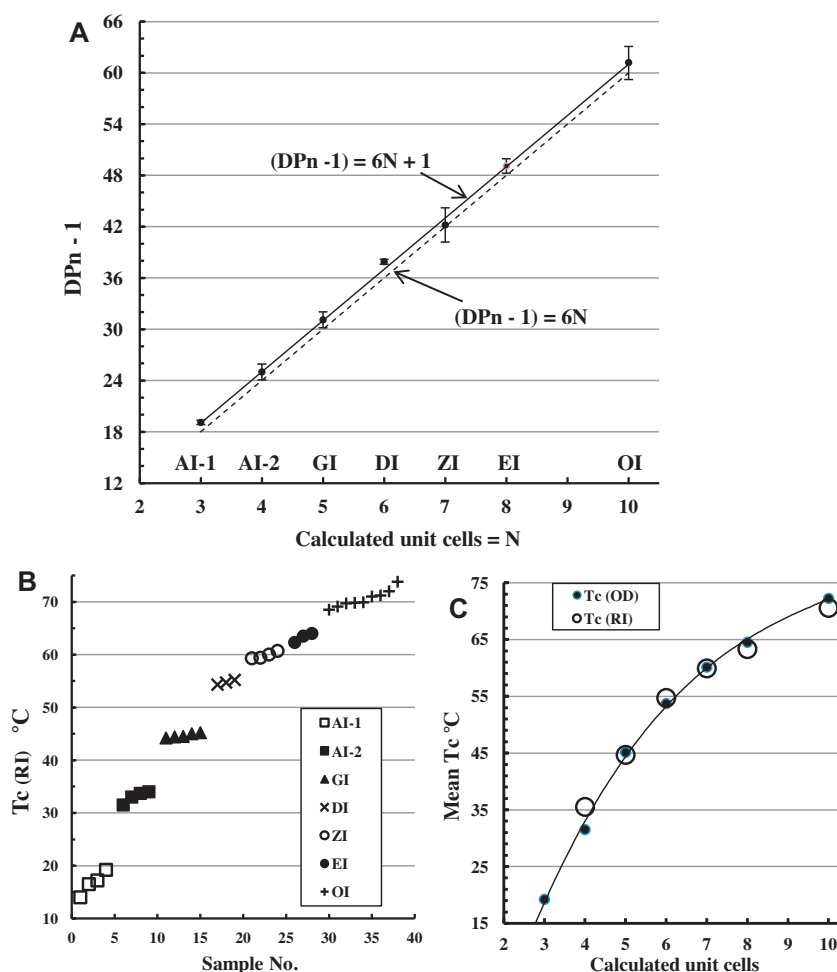
Fig. 2. Relation of DPn to monoformat isoform type (Table 2). (A) Mean (DPn - 1) values plotted against isoform type and unit cells calculated as DPn/6 (nearest integer). Error bars show ± standard error. The dashed line shows the expected progression 6N, while the solid line shows the linear trend line (MS Excel™ 2007) of the observed (DPn - 1) progression. (B) Tc (RI) values of the monoformat preparations arranged in increasing order. (C) Mean Tc plotted against calculated unit cells.
