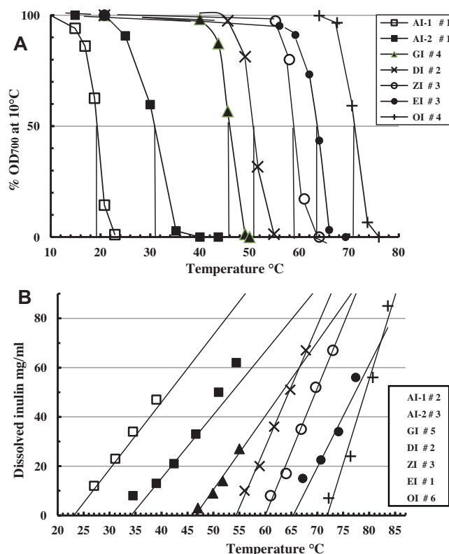
Fig. 1. Comparisons of thermal properties of typical monoformat isoform isolates satisfying the monoformat criteria, showing conformity with the plus-format series (Cooper et al., 2013b). (A) \text{OD}_{700} thermal transition curves. Dilutions in PBS at 0.5\ \text{mg mL}^{-1} are progressively heated and the \text{OD}_{700} of each measured after equilibration at each indicated temperature. (B) Temperature solubility curves. Sealed Eppendorf centrifuge tubes containing 0.5\ \text{mL} of isoform suspensions at 50 – 100\ \text{mg mL}^{-1} are fully immersed in water baths at the indicated temperatures for 15 min and then centrifuged (4 min, 18,000 \times g ) to measure supernatant RI. The linear trend-lines created by the application (MS Excel 2007 TM ) are extrapolated to zero supernatant content. Legends show sample numbers of Table 2.
